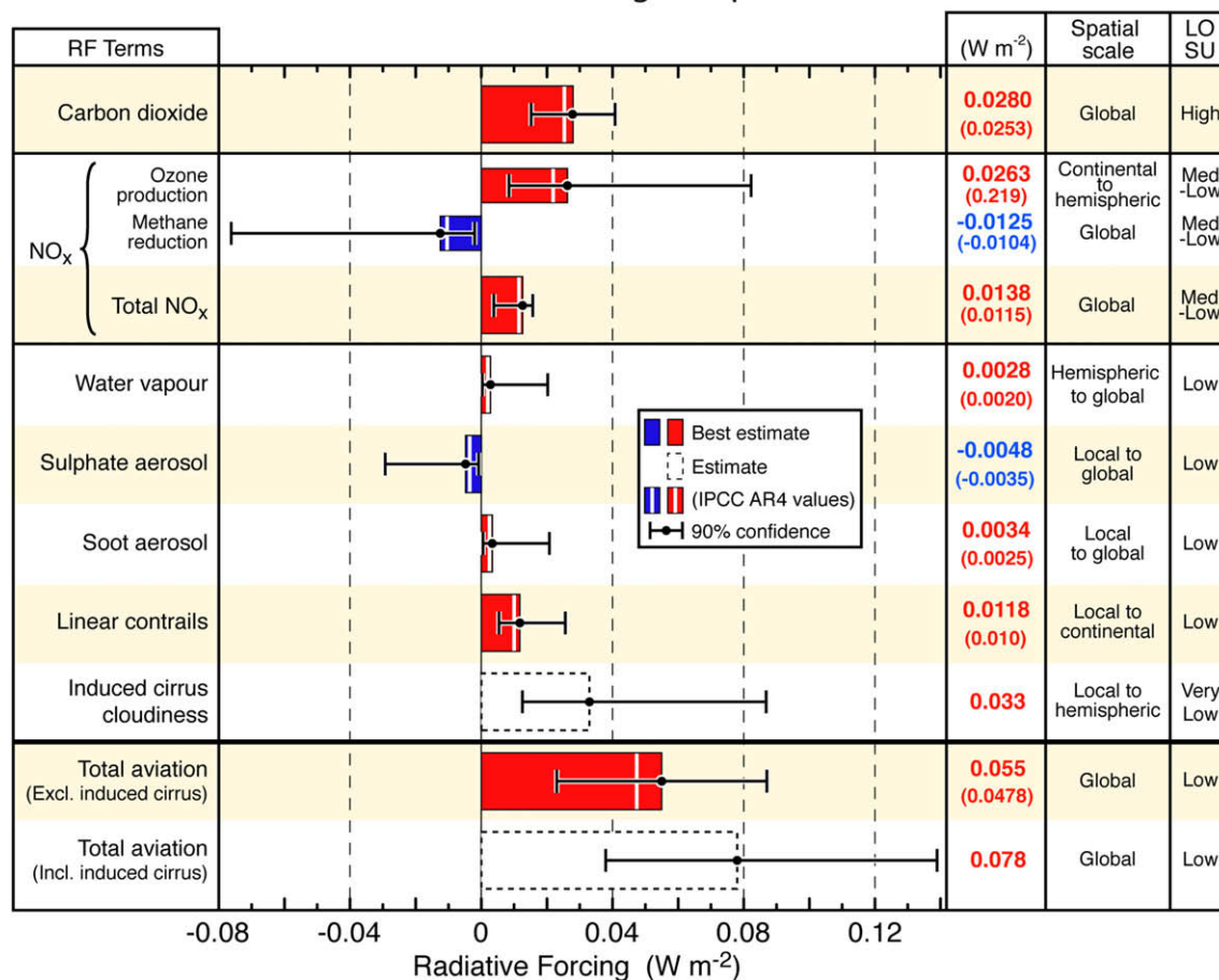
Fig. 4. Radiative forcing components from global aviation as evaluated from preindustrial times until 2005. Bars represent updated best estimates or an estimate in the case of aviation-induced cloudiness (AIC) as listed in Table 2. IPCC AR4 values are indicated by the white lines in the bars as reported by Forster et al. (2007a). The induced cloudiness (AIC) estimate includes linear contrails. Numerical values are given on the right for both IPCC AR4 (in parentheses) and updated values. Error bars represent the 90% likelihood range for each estimate (see text and Tables 2 and 3). The median value of total radiative forcing from aviation is shown with and without AIC. The median values and uncertainties for the total NO x RF and the two total aviation RFs are calculated using a Monte Carlo simulation (see text). The Total NO x RF is the combination of the CH 4 and O 3 RF terms, which are also shown here. The AR4 value noted for the Total NO x term is the sum of the AR4 CH 4 and O 3 best estimates. Note that the confidence interval for 'Total NO x ' is due to the assumption that the RFs from O 3 and CH 4 are 100% correlated; however, in reality, the correlation is likely to be less than 100% but to an unknown degree (see text). The geographic spatial scale of the radiative forcing from each component and the level of scientific understanding (LOSU) are also shown on the right.
